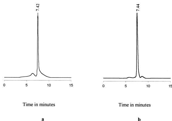
Figure 1. Reverse phase HPLC of d(AT). (a) Synthesized on PEG support by nucleoside \beta -CE-H-phosphonate approach. (b) Synthesized on solid phase by phosphoramidite approach.
