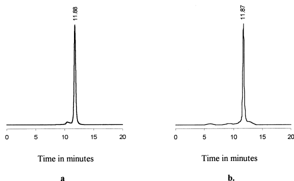
Figure 2. Reverse phase HPLC of d(ACGGGCCCCGT). (a) Synthesized on PEG support by nucleoside \beta -CE-H-phosphonate approach. (b) Synthesized on solid phase by phosphoramidite approach.
